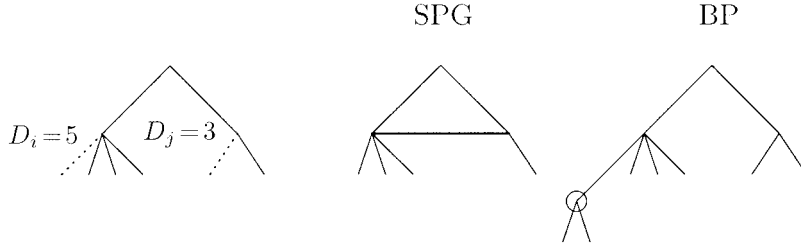
Fig. 4. Example of the coupling when a cycle occurs. Edges have twice the length of stubs. In the SPG the two dotted stubs in the left picture are to be connected. The middle picture gives the result of creating the cycle in the SPG where the bold line is the edge creating the cycle. The third figure draws the BP where the cycle is removed and the degree of the circled node is 3.
