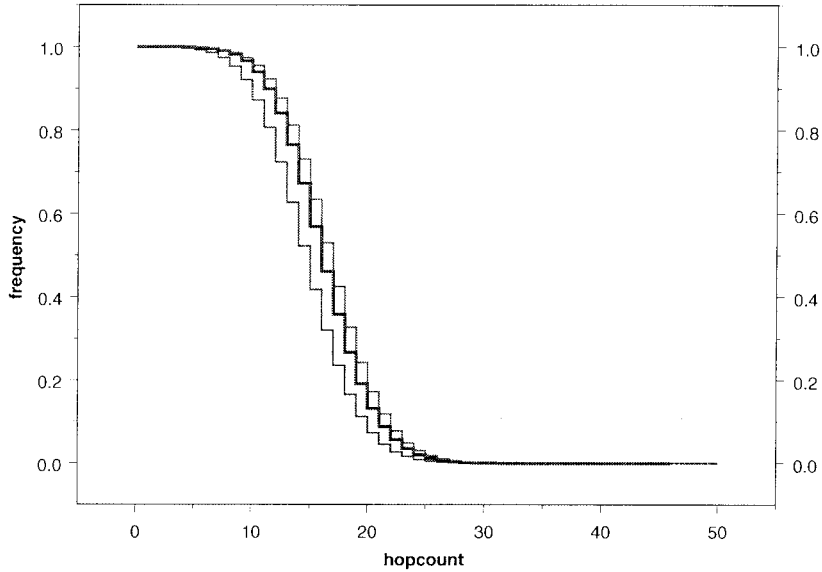
Fig. 1. Empirical survival functions of the hopcount for \tau = 3.5 and the values N = 25,000 , N = 75,000 (bold), and N = 125,000 , based on samples of size 1,000.
