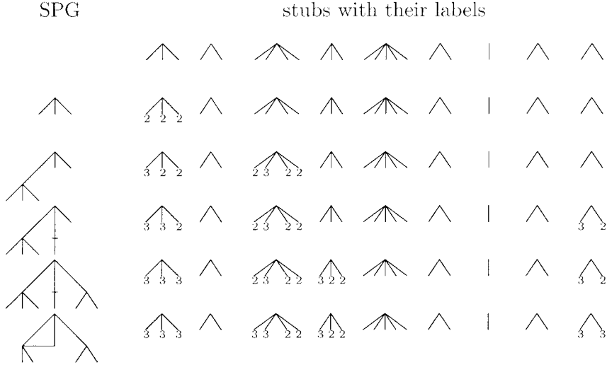
Fig. 3. Schematic drawing of the growth of the SPG from the node 1 with N = 9 and the updating of the labels. The stubs without labels have label 1. The first line shows the N different degrees. The growth process starts by choosing the first stub of node 1 whose stubs are labeled by 2 as illustrated in the second line, while all the other stubs maintain the label 1. Next, we uniformly choose a stub with label 1 or 2. In the example in line 3, this is the second stub from node 3, whose stubs are labeled by 2 except for the second stub which is labeled 3. The left-hand side column visualizes growth of the SPG by the attachment of stub 2 of node 3 to the first stub of node 1. Once an edge is established, the paired stubs are labeled 3. In the next step, the next stub of node one is again matched to a uniform stub out of those with label 1 or 2. In the example in line 4, it is the first stub of the last node that will be attached to the second stub of node 1, the next in sequence to be paired. The last line exhibits the result of creating a cycle when the first stub of node 3 is chosen to be attached to the last stub of node 9 (the last node). This process is continued until there are no more stubs with labels 1 or 2. In this example, we have Z_1^{(1)} = 3 and Z_2^{(1)} = 6 .
