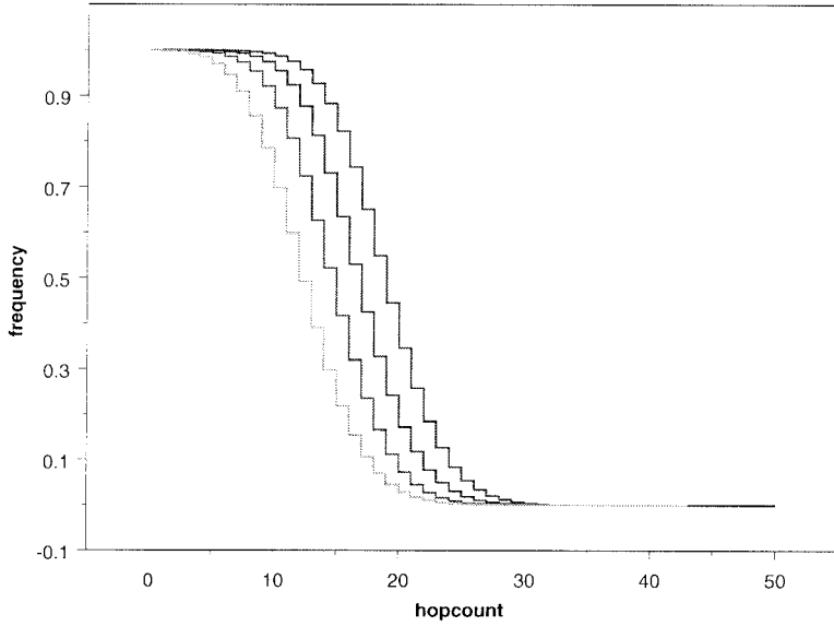
Fig. 2. Empirical survival functions of the hopcount for \tau = 3.5 and the four values N_k = 5000v^{2k} , k = 0, 1, 2, 3 , based on 1000 runs.
