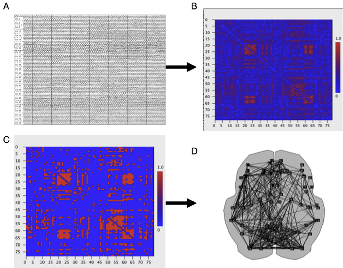
Fig. 1. Schematic illustration of graph theoretical analysis of multi channel MEG data. (A) The starting point is a multi channel recording of brain activity, either EEG or MEG, filtered in a frequency band of interest. The same approach can be used for fMRI BOLD time series. (B) A measure of correlation or synchronization is computed between all possible pairs of channels. The results are shown in a N by N matrix, where each entry contains the correlation or synchronization strength of a particular pair of channels. In this case the magnitude of the synchronization is shown on a colour scale from 0 (blue) to 1 (red). (C) After application of a threshold T all cells with a value larger than T are given a value of 1, and all other cells a value of 0. This step converts the weighted complete graph to a binary graph. In this case the original matrix is symmetrical and the resulting graph is undirected. (D) The binary graph is shown in a glass brain representation. Each node corresponds to a recording site or MEG source, and nodes are connected by an edge if the synchronization strength exceeds the threshold T . From this graph various graph theoretical measures such as the clustering coefficient and the average shortest path length can be computed.
