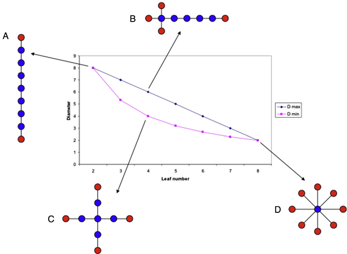
Fig. 3. Schematic illustration of trees and tree measures. Different configurations of a tree consisting of N = 9 nodes and m = 8 edges. The plot in the middle shows the diameter (maximum distance between any two edges of the tree) as a function of the leaf number (number of nodes with only one edge). Leaf nodes are shown in red. All other nodes are blue. D_{\max} represents the highest possible diameter for a tree with a given leaf number L . D_{\max} = N - L + 1 . D_{\min} represents the lowest possible diameter for a tree with a given leaf number L : D_{\min} = 2(N - 1) / L . (A) tree with L = 2 and D_{\max} = D_{\min} = 8 . This type of tree is called a path. (B) Tree with the longest possible diameter (6) for a leaf number of 4. (C) Tree with the lowest possible diameter (4) for a leaf number of 4. (D) Tree with diameter of 2 and leaf number of 8. This type of tree is called a star. The path and the tree represent two extreme configurations of a tree. The area between the lines corresponding to D_{\max} and D_{\min} represent a space of different possible tree configurations, bounded by maximum and minimum possible diameter for each leaf number.
