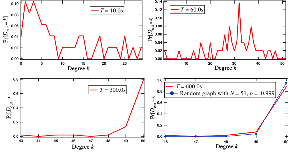
Fig. 3: Topology evolution of the neighbor graph as a function of time series. The outgoing degree defines the number of neighboring connections a node once maintained. In the bottom-right sub-figure, \Pr[D_{out} = k] is fitted with the degree distribution of a random graph with link density p = 0.999 .
