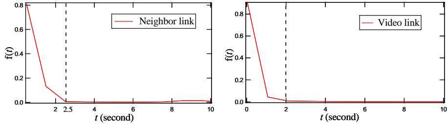
Fig. 2: Pdf of the activation period of the neighbor link (left) and the video link (right). Threshold of activation period for the neighbor link is \tau_N \sim 2.5 s, and \tau_V \sim 2.0 s for the video link.
