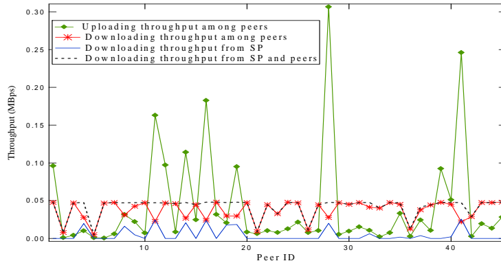
Fig. 7: Uploading and downloading throughput at every SopCast node during the entire experiment (40 minutes). The x -axis presents the identification number (ID) of each individual peer. The uploading throughput (downloading throughput) at a single peer is calculated based on the amount of data uploads (downloads) to all the children (parents) the peer has.
