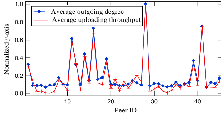
Fig. 8: Correlation between the average outgoing degree and the average uploading throughput with the snapshot duration of 2.0 seconds. The y -axis is normalized by y^* = \frac{y}{y_{\max}} .
