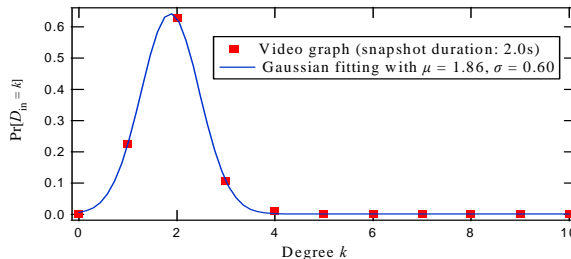
Fig. 5: Pdf of the incoming degree (number of parents) of the video graph on a linear scale. Snapshot duration of the video graph is set to 2.0 s. A Gaussian fitting describes the pdf of D_{in} well, which suggests us to model the incoming degree of G_V as a random graph with very low link density p \ll 1.0 .
