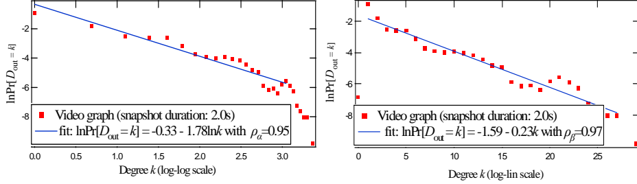
Fig. 6: The outgoing degree (number of children) distribution of the G_V on both log-log scale (left) and log-lin scale (right). The linear correlation coefficients \rho_\alpha on the log-log scale and \rho_\beta on the log-lin scale are used to reflect the fitting quality.
