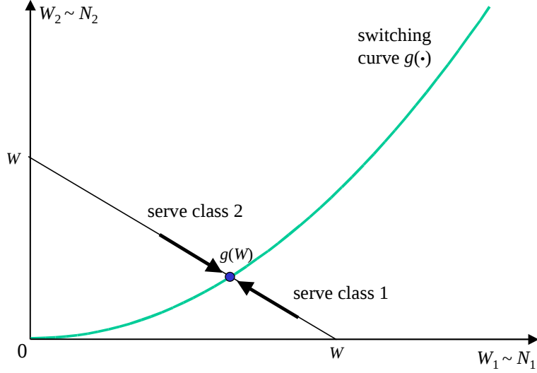
Figure 1: The switching curve g(\cdot) defines the dynamic Gc\mu scheduling rule.
